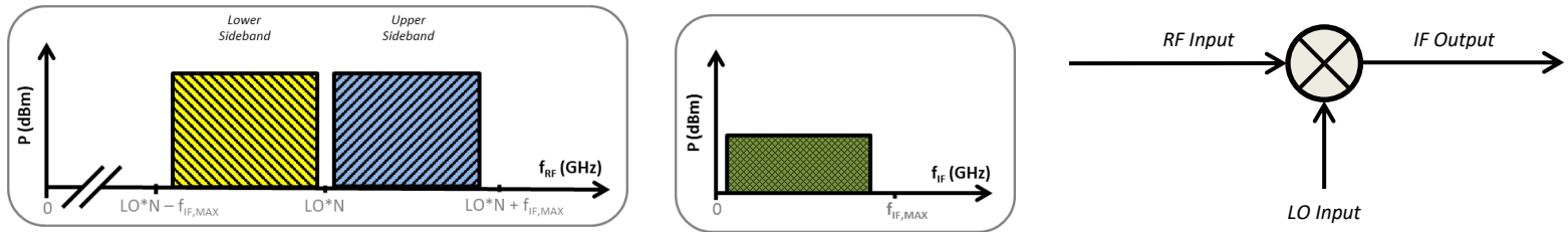
Figure 2: Diagram of block down-conversion is shown.
