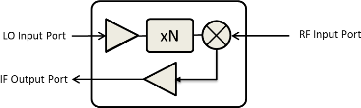
Figure 1: MixAMC-I Block Diagram Simplified block diagram for a typical MixAMC-I module is shown. Location of power amplifiers and multipliers vary for each unit. N is the harmonic factor for this configuration. The standard MixAMC-I configuration comes with an integrated IF amplifier. The MixAMC-I can be configured without the IF amplifier (part number: MixAMC-I-N), allowing for direct access to the mixer IF port.
